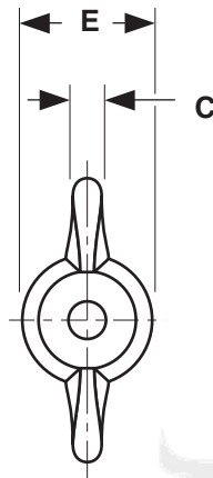
WING NUTS - COLD FORGED (TYPE-A)
