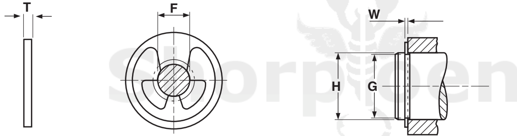
TYPE E RETAINING RINGS
