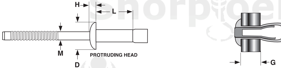
STRUCTURAL RIVETS WITH PROTRUDING HEADS
