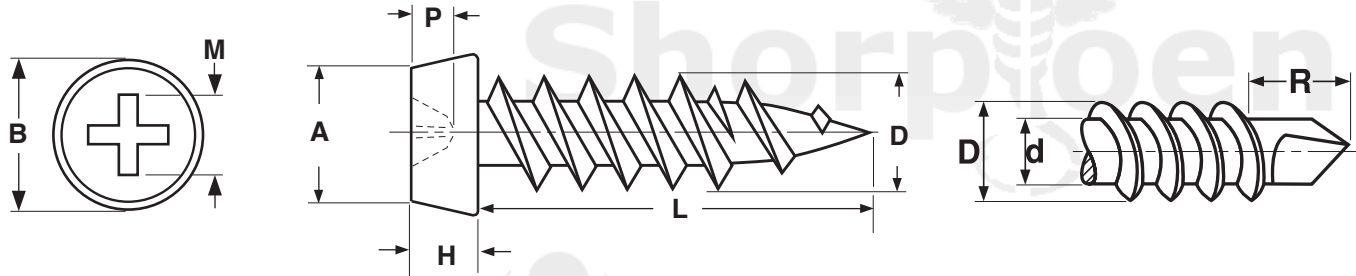
PAN PHILLIPS FRAMING SCREW — SHARP POINT
