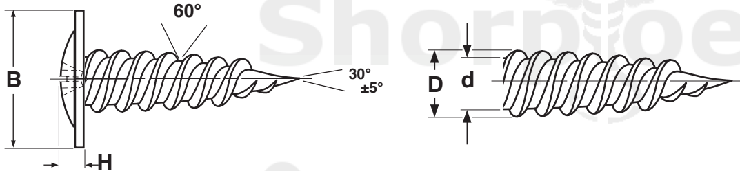
MODIFIED TRUSS PHILLIPS SELF-PIERCING SCREWS
